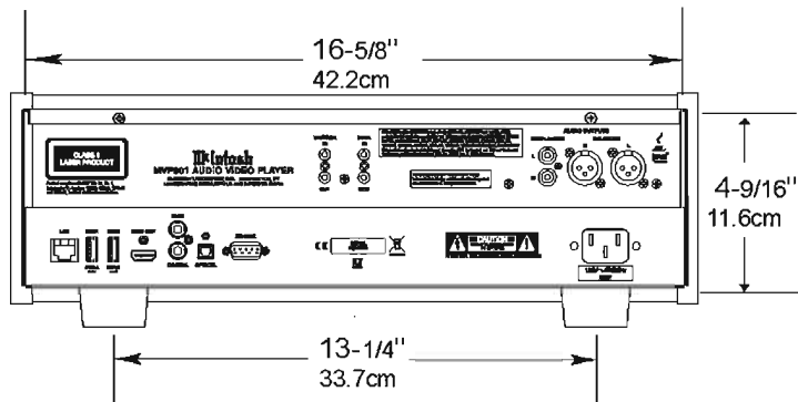
Rear View of the MVP901
