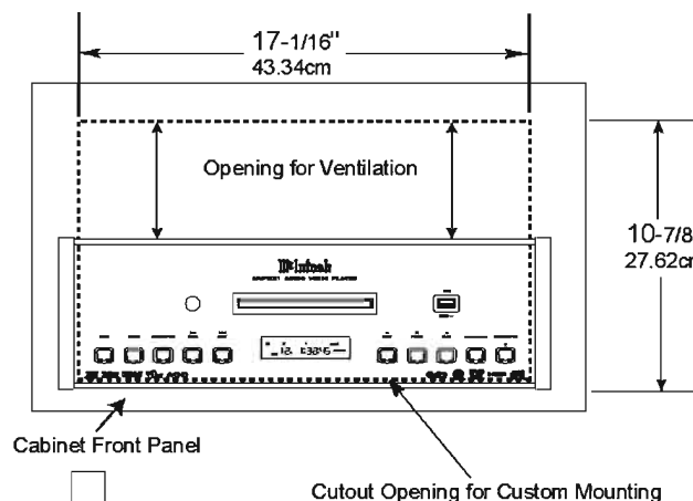
MVP901 Front Panel Custom Cabinet Cutout
