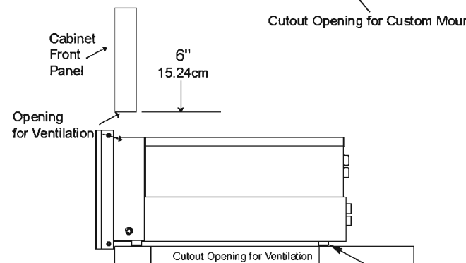
MVP901 Side View in Custom Cabinet
