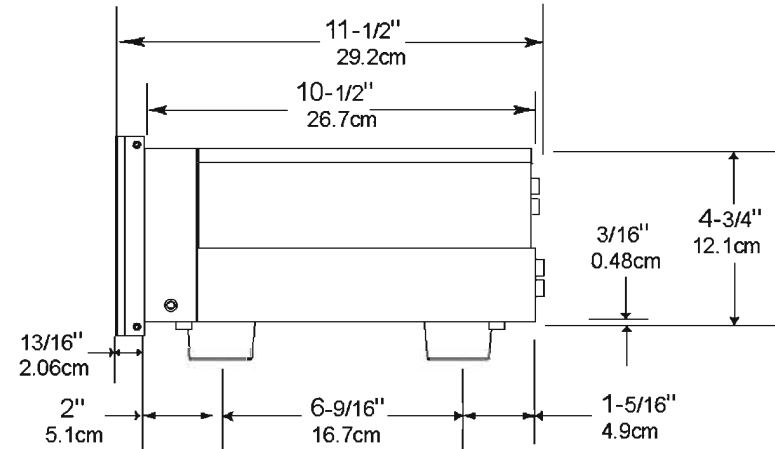
Side View of the MVP901
